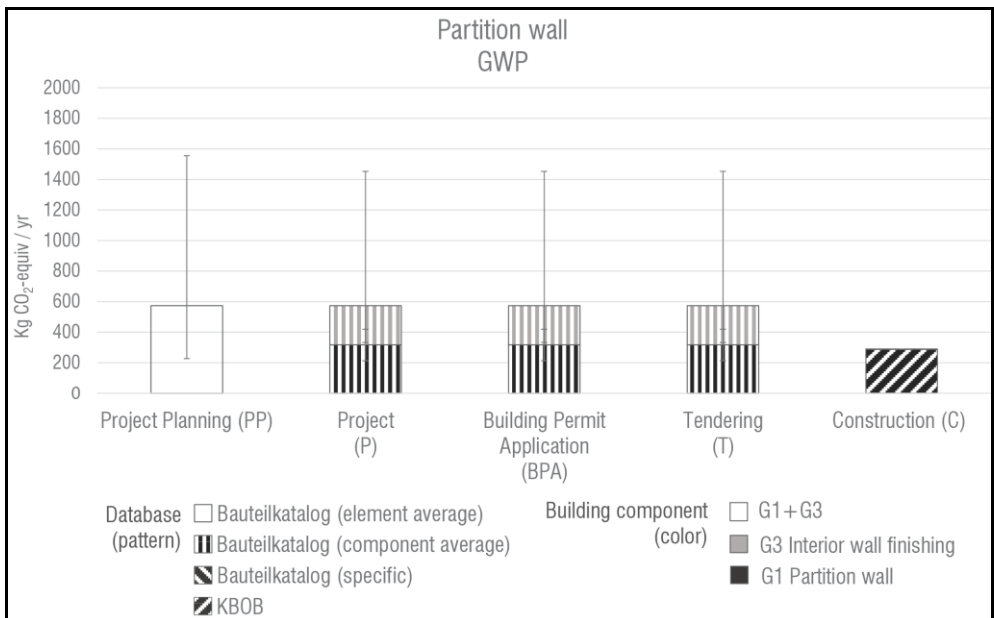
Fig. 30 – Contribution to the GWP of Partition wall during the design process
