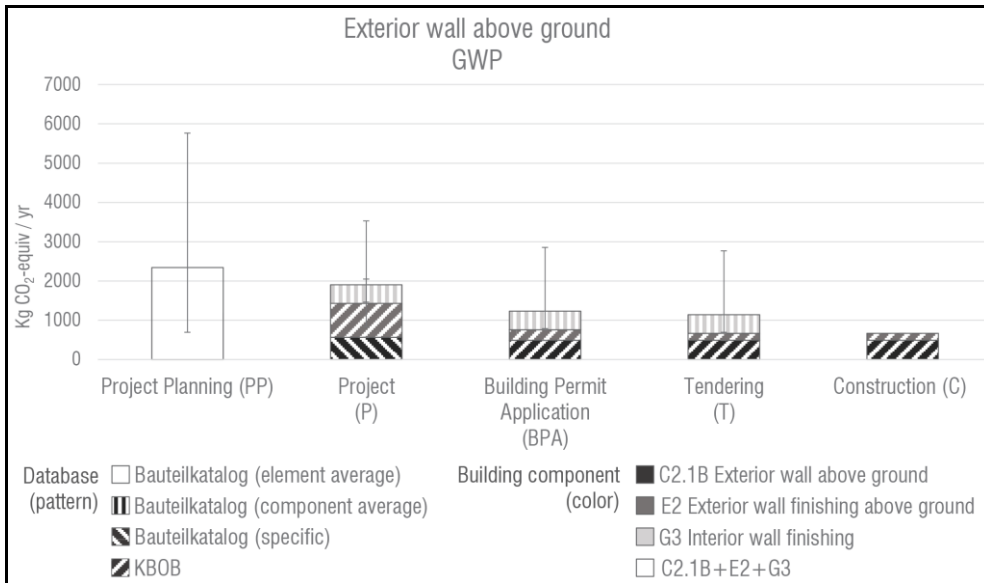
Fig. 27 – Contribution to the GWP of External wall above ground during the design process
